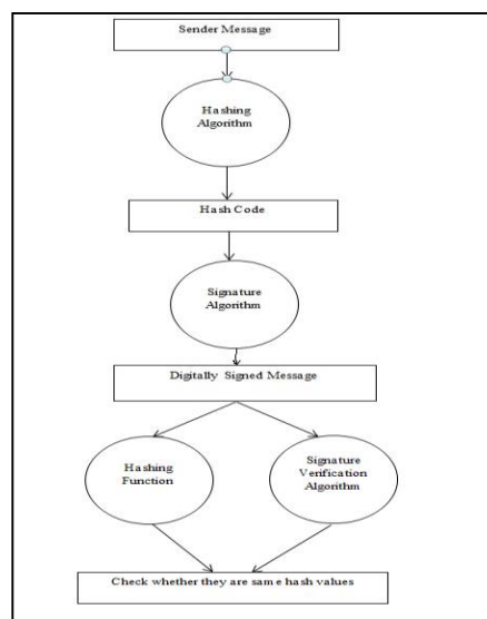
Fig. 5. Signing and Verification of Digital Signatures.
