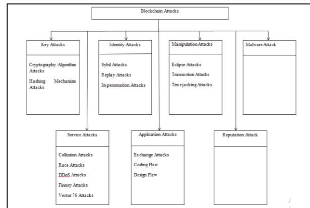
Fig. 7. Various Blockchain Security Attacks.
