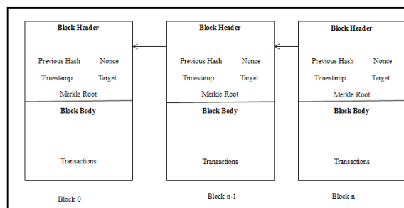
Fig. 4. Structure of a Block.
