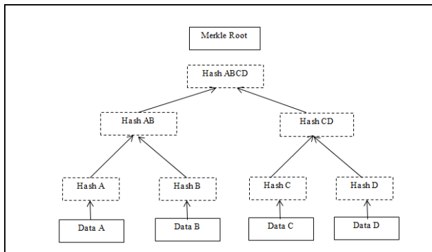
Fig. 6. Representation of a Merkle Tree.
