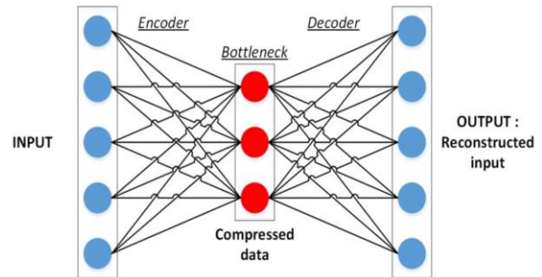
Fig. 10. Autoencoder's Model.
