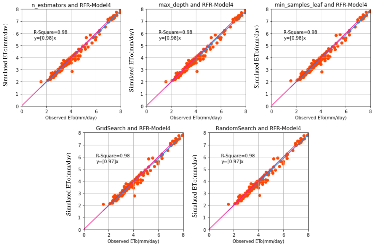
Fig. 5. Regression Analysis of the RFR-Model4 in all Scenarios.
