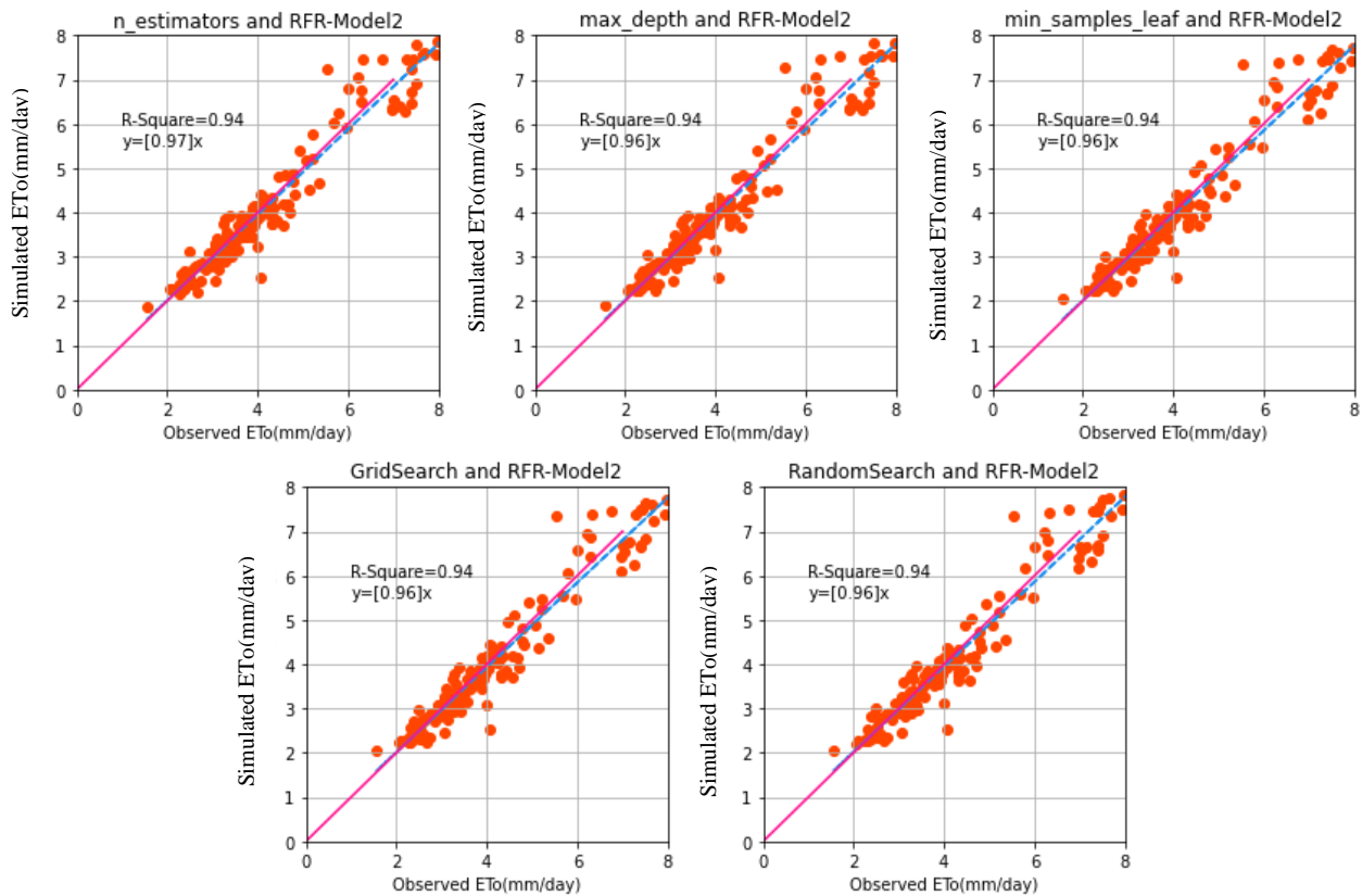
Fig. 3. Regression Analysis of the RFR-Model2 in all Scenarios.
