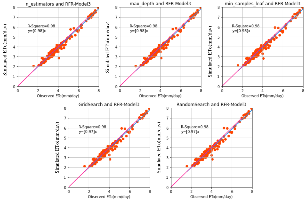
Fig. 4. Regression Analysis of the RFR-Model3 in all Scenarios.
