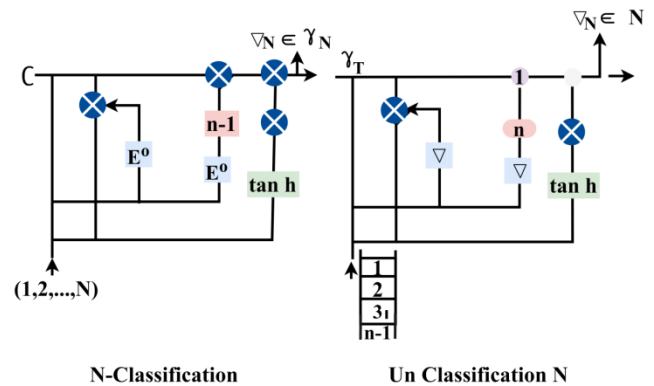
Fig. 2. Classification Process.
