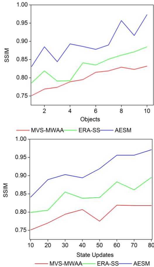
Fig. 6. SSIM Analysis.
