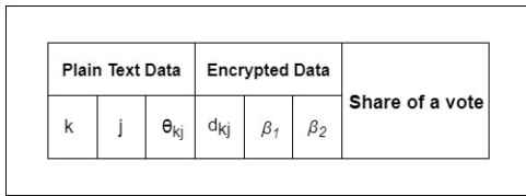
Fig. 1. The pair table data layout stores in the cloud. Each row of the pair table data contains plain text data ( k, j, \theta_{kj} ), encoding data ( d_{kj} , \beta_1 , \beta_2 ) and share of vote
