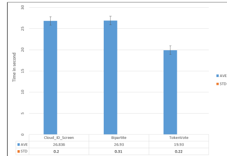
Fig. 3. The speed result comparing the performance of our TokenVote scheme against the two baselines
