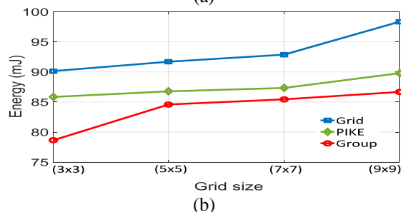
Fig. 6. Average energy consumed by the nodes of the four schemes for (a) Random subset assignment KPDS, (b) Grid-based KPDS, PIKE and group-based KPDS.
