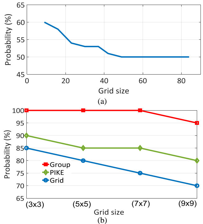
Fig. 8. Probability of establishing an indirect key between two nodes for (a) Random subset assignment KPDS, (b) Grid-based KPDS, PIKE and group-based KPDS.
