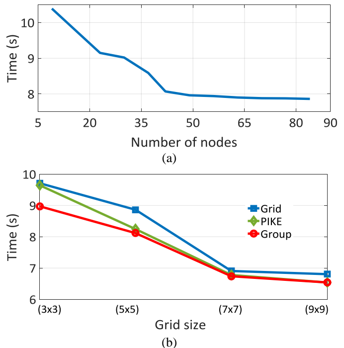
Fig. 4. Time for establishing a session for (a) Random subset assignment KPDS, (b) Grid-based KPDS, PIKE and group-based KPDS.
