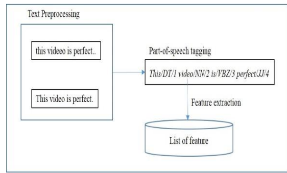
Fig. 2. Text Preprocessing
